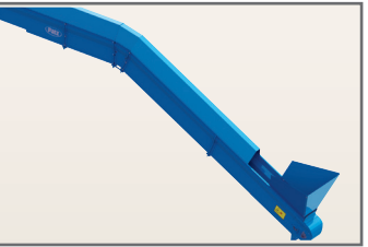
22 ½° and 7 ½° decline elbows available. Fasten two 7 ½° elbows together to form 15°.
