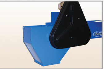
Short spout assembly attaches on front end of conveyor.
