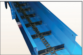
Detachable Steel Chain with 1 ½" high steel flites and 12" spacing delivers high capacity.
