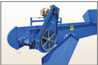
Motor mounts to top or bottom of conveyor. This unit uses a single V-belt with roller chain reduction. Note: Guarding removed for viewing.
