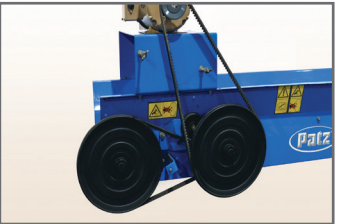
Easy Maintenance. All belt drive makes maintenance easy. Greasable bearing provide long life. Note: Guarding removed for viewing.
