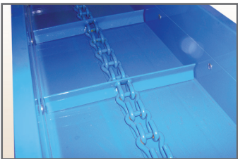
Heat-treated, heavy-duty, double-hook links are welded to 2" x 15 ½" steel flites. Flite spacing is 14 ½". Links are detachable without tools for easy service.
