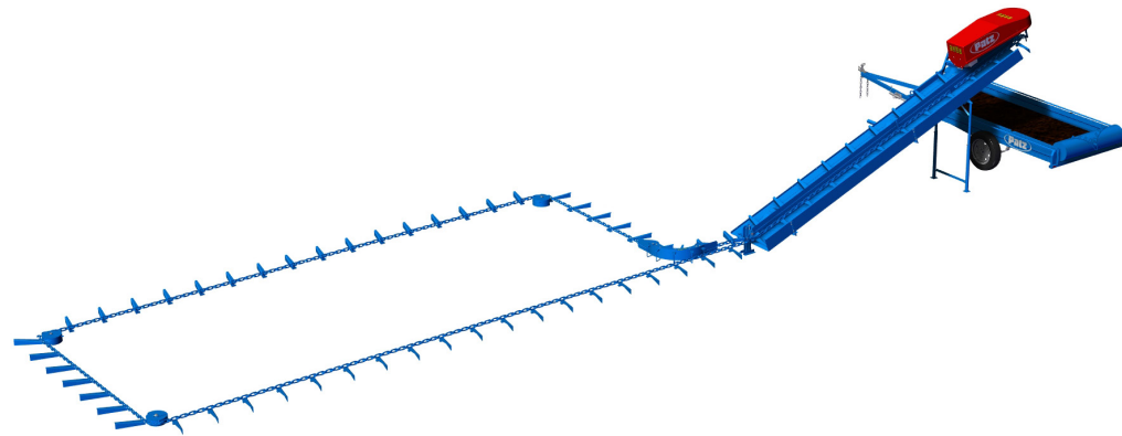
Continuous Loop, Multi-Gutter Barn Cleaner that Conveys Manure Up an Elevated Slide and Drops the Manure into a Manure Spreader with the Flip of a Switch
